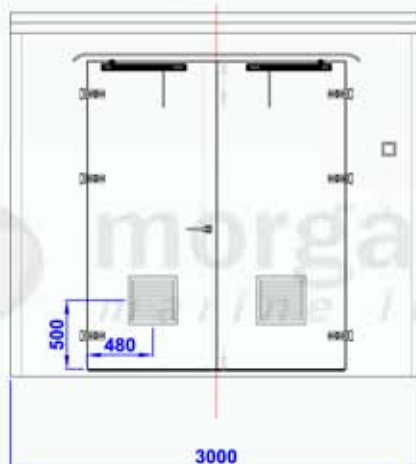
EXTERNAL ELEVATION WALL 1
